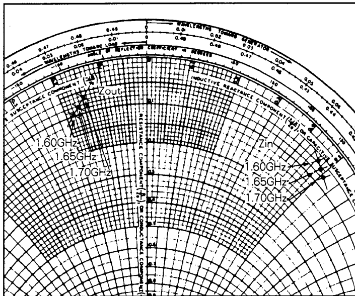
INPUT AND OUTPUT SERIES IMPEDANCE 2SC4838
